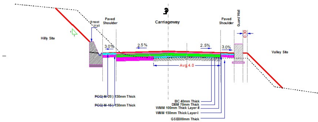
TYPICAL CROSS SECTION – III E
