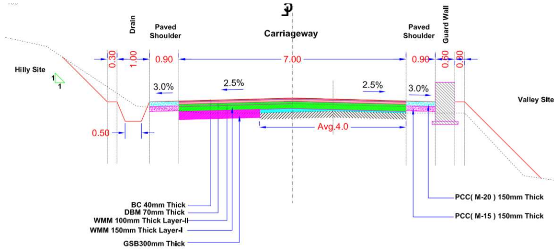
TYPICAL CROSS SECTION – III D
