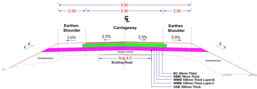
TYPICAL CROSS SECTION – II B
