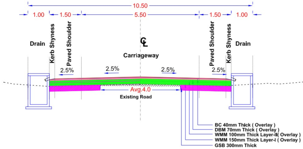
TYPICAL CROSS SECTION – I A
